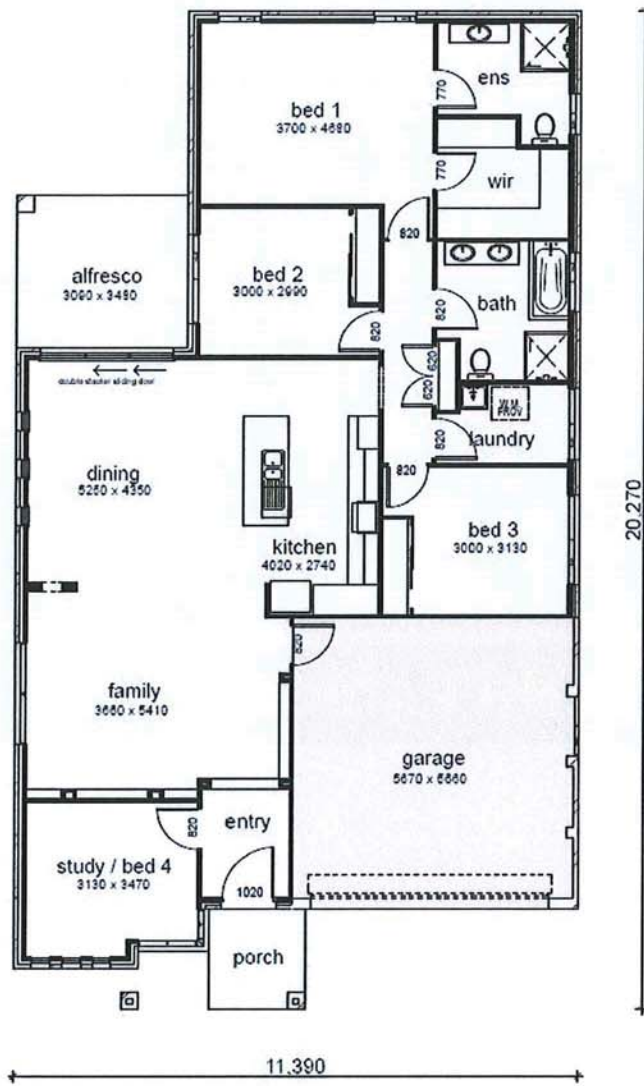
Floor Plan
